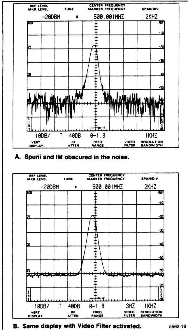
Figure 6-5. Typical display mixed with the VIDEO FILTER.
